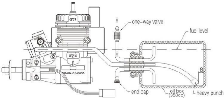
Oil-box installation schemes
